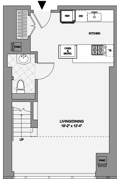
LOWER LEVEL
